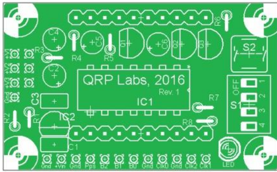
PCB 48 x 29mm
