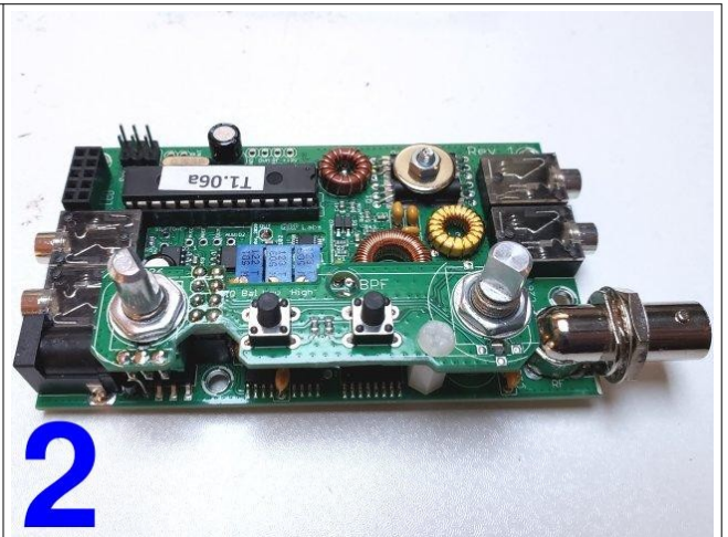
... and the main board, with the controls board bolted in position.
