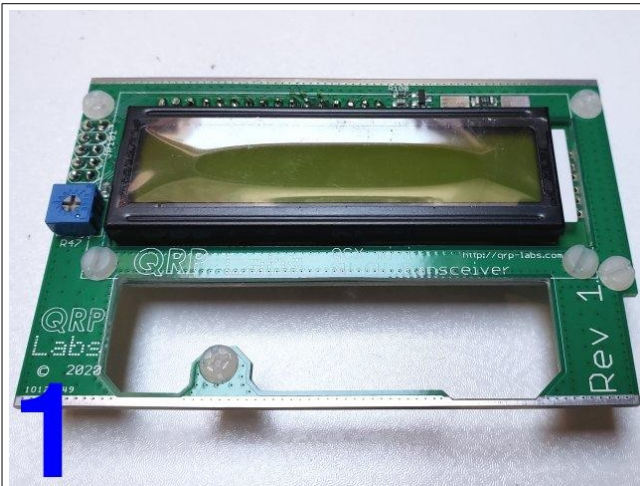
Start with the Display board...
