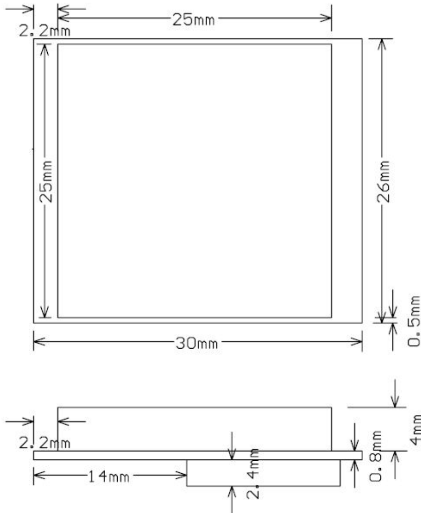
Figure 3: SKM61 Dimensions
