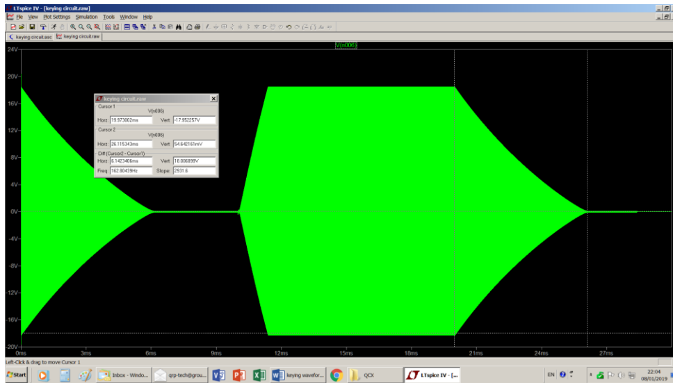
R41 - 470 ohms, BF = 250, C31 = 1 ufd Risetime = 1.3 milliseconds, Fall time = 6.1 milliseconds
