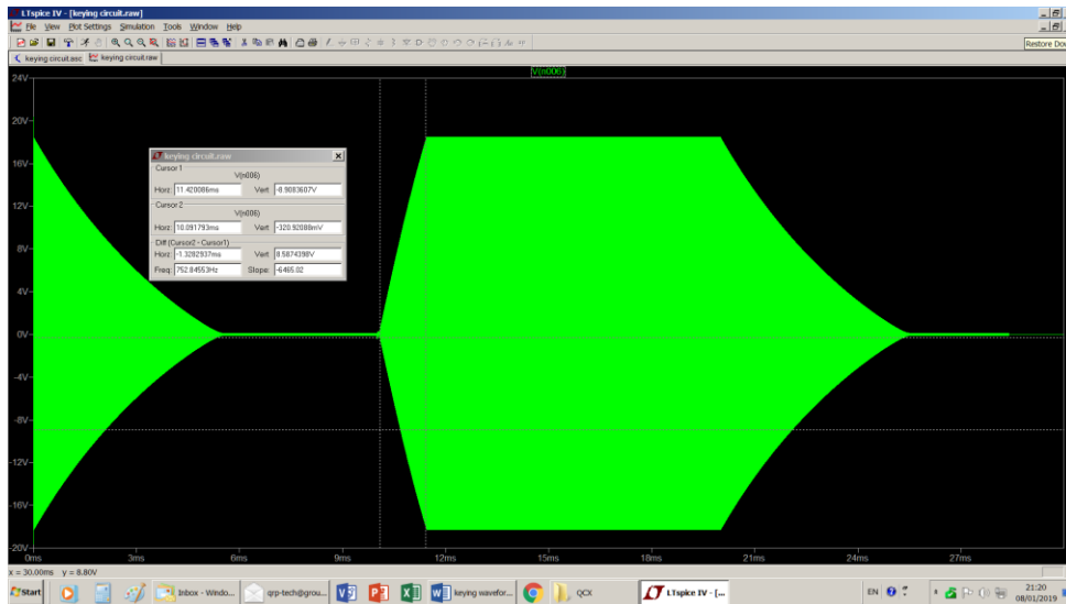
R41 - 470 ohms, BF = 170, C31 = 1 ufd Risetime = 1.3 milliseconds, Fall time = 5.5 milliseconds
