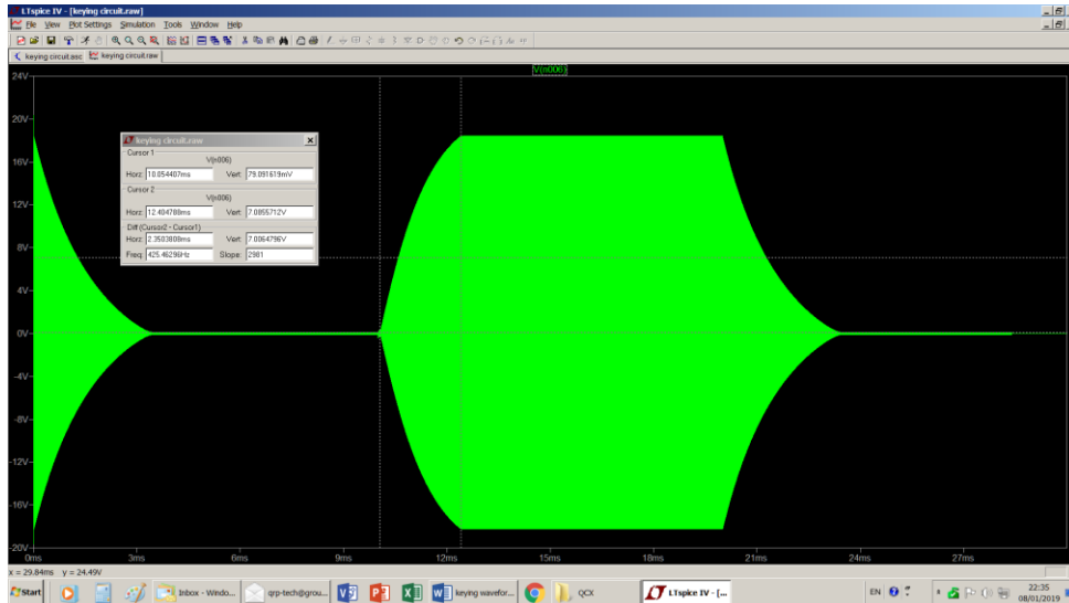
R41 - 470 ohms, BF = 50, C31 = 1 ufd Risetime = 2.3 milliseconds, Fall time = 3.3 milliseconds
