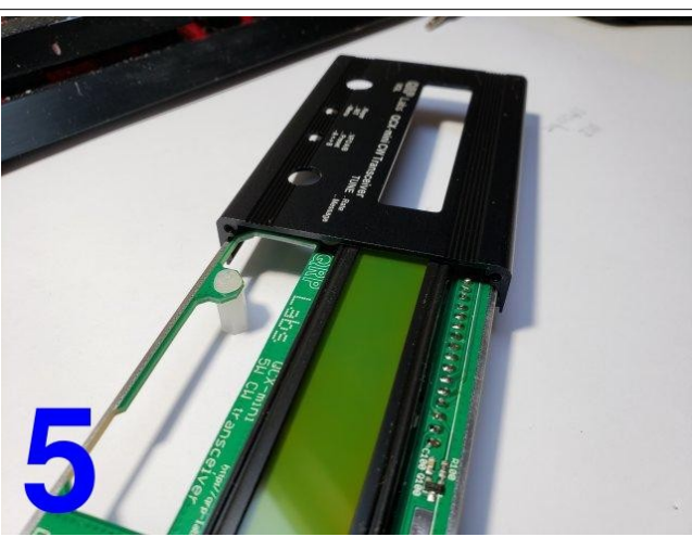
Slide the display board into position along the PCB guide rails in the enclosure.
