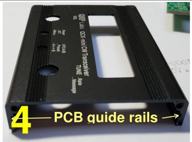
Here's the top half of the enclosure. Note the PCB guide rails in the extrusion walls.
