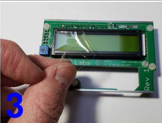
Peel off the plastic protective coating from the LCD module.
