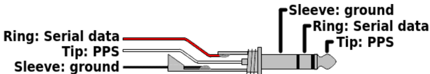
Paddle connector, used for GPS
