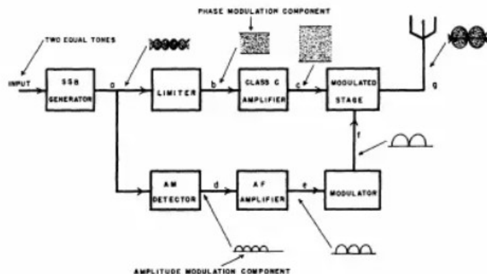
Fig. 2—Simplified block diagram of system.
